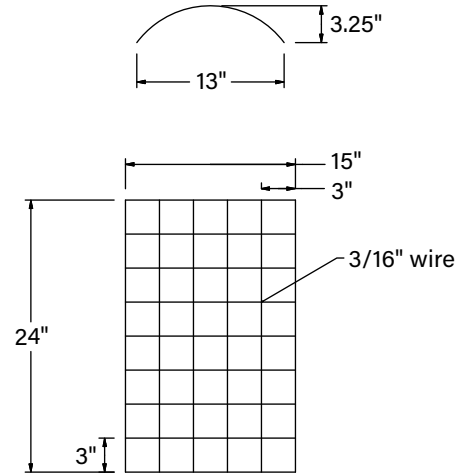
Safety Cage
