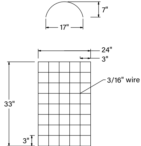
Safety Cage
