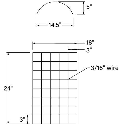
Safety Cage
